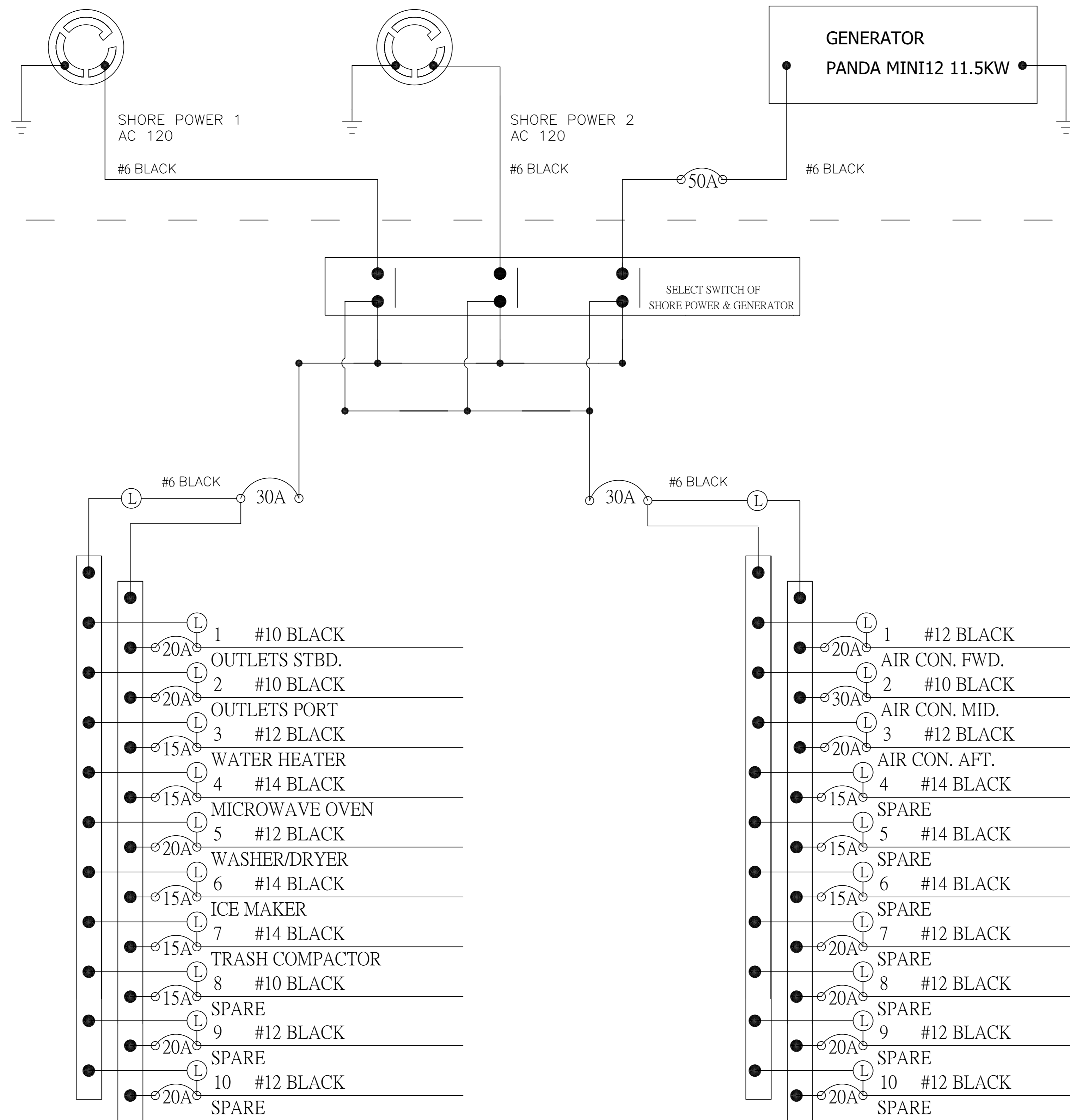
MAIN SWITCH BOARD NEWMAR ES-5
